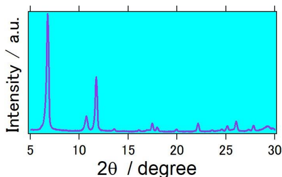
XRD of GS MOF Cu-74
